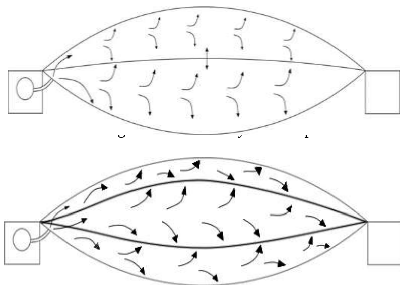
Figure 1. Four-layer ETFE pillow
